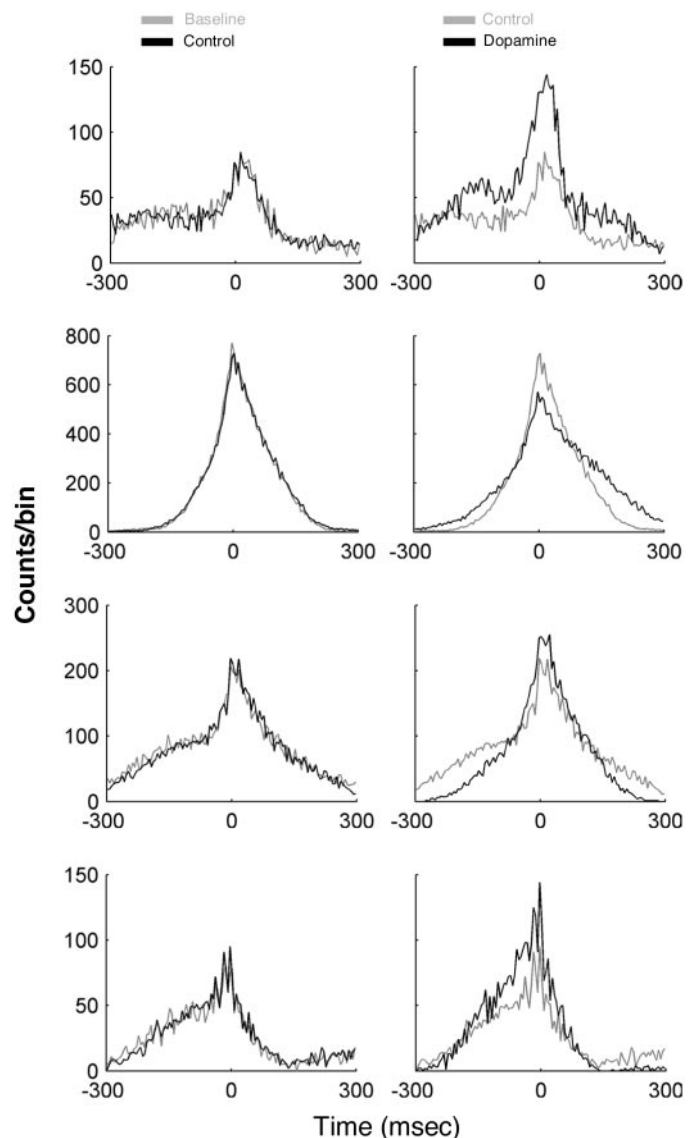
FIG. 3. Cross-correlograms of 4 different pairs of electrodes are shown. Left : cross-correlograms in the baseline (gray) and control (black) phases. Right : for the same electrode pairs, cross-correlograms in the control (gray, same correlogram as in the left ) and dopamine phase (black). Bin size is 5 ms. Electrode pairs were chosen from 3 different experiments.
