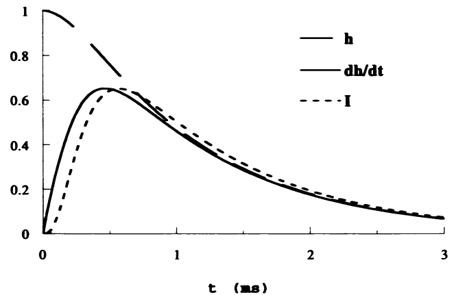
FIGURE 4 Inactivation delay in the state-dependent model. The inactivation variable h and its rate of change dh/dt are plotted against time after a rapid depolarization (at t = 0 ) to +10 mV from a holding potential of -100 mV. The short-dashed curve is the total sodium current normalized so that its height matches that of dh/dt . For h , the y axis is in dimensionless units; for dh/dt , the y axis is in units of 1/\text{ms} , for I , it is in arbitrary units of current. This figure demonstrates that the inactivation process is delayed, but the delay is less than that of the full current. Compare with Fig. 11 of Bean (1981).
