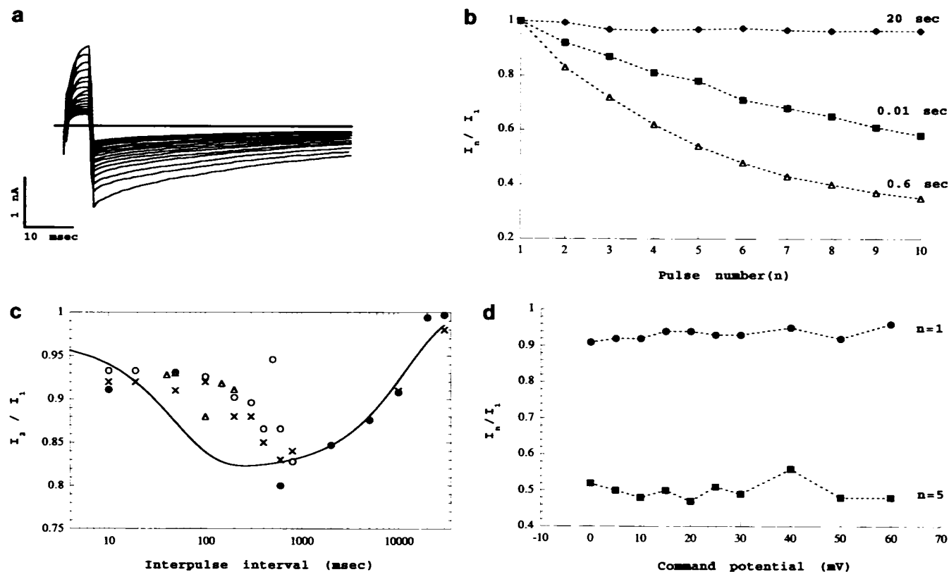
FIGURE 1 Cumulative inactivation of Kv3. ( a ) Superposition of current traces evoked by a series of 20 5 ms duration pulses to +40 mV, separated by interpulse intervals of 50 ms at -80 mV. ( b ) Frequency dependence of cumulative inactivation. The ratio of the peak current amplitude during each pulse, relative to that during the 1st pulse, is plotted against the pulse number ( n ) at three different interpulse intervals (next to each curve). Holding voltage -100 mV, interpulse voltage -80 mV, pulse duration 10 ms. ( c ) Biphasic recovery from inactivation. I_2/I_1 at different inter-pulse intervals from four different patches. Note the logarithmic time scale. The solid line is the prediction of the final model, which is presented and discussed later in the text. ( d ) Rate of cumulative inactivation is independent of membrane potential during the pulse, as measured by the ratio of I_2/I_1 and I_3/I_1 at several fully activating voltages. Interpulse interval 30 ms, pulse duration 30 ms, holding potential between pulses and pulse series is -100 mV.
