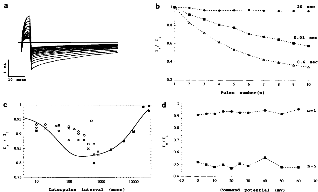
FIGURE 1 Cumulative inactivation of Kv3. (a) Superposition of current traces evoked by a series of 20 5 ms duration pulses to +40 mV, separated by interpulse intervals of 50 ms at -80 mV. (b) Frequency dependence of cumulative inactivation. The ratio of the peak current amplitude during each pulse, relative to that during the 1st pulse, is plotted against the pulse number ( n ) at three different interpulse intervals (next to each curve). Holding voltage -100 mV, interpulse voltage -80 mV, pulse duration 10 ms. (c) Biphasic recovery from inactivation. I_2/I_1 at different inter-pulse intervals from four different patches. Note the logarithmic time scale. The solid line is the prediction of the final model, which is presented and discussed later in the text. (d) Rate of cumulative inactivation is independent of membrane potential during the pulse, as measured by the ratio of I_2/I_1 and I_3/I_1 at several fully activating voltages. Interpulse interval 30 ms, pulse duration 30 ms, holding potential between pulses and pulse series is -100 mV.
