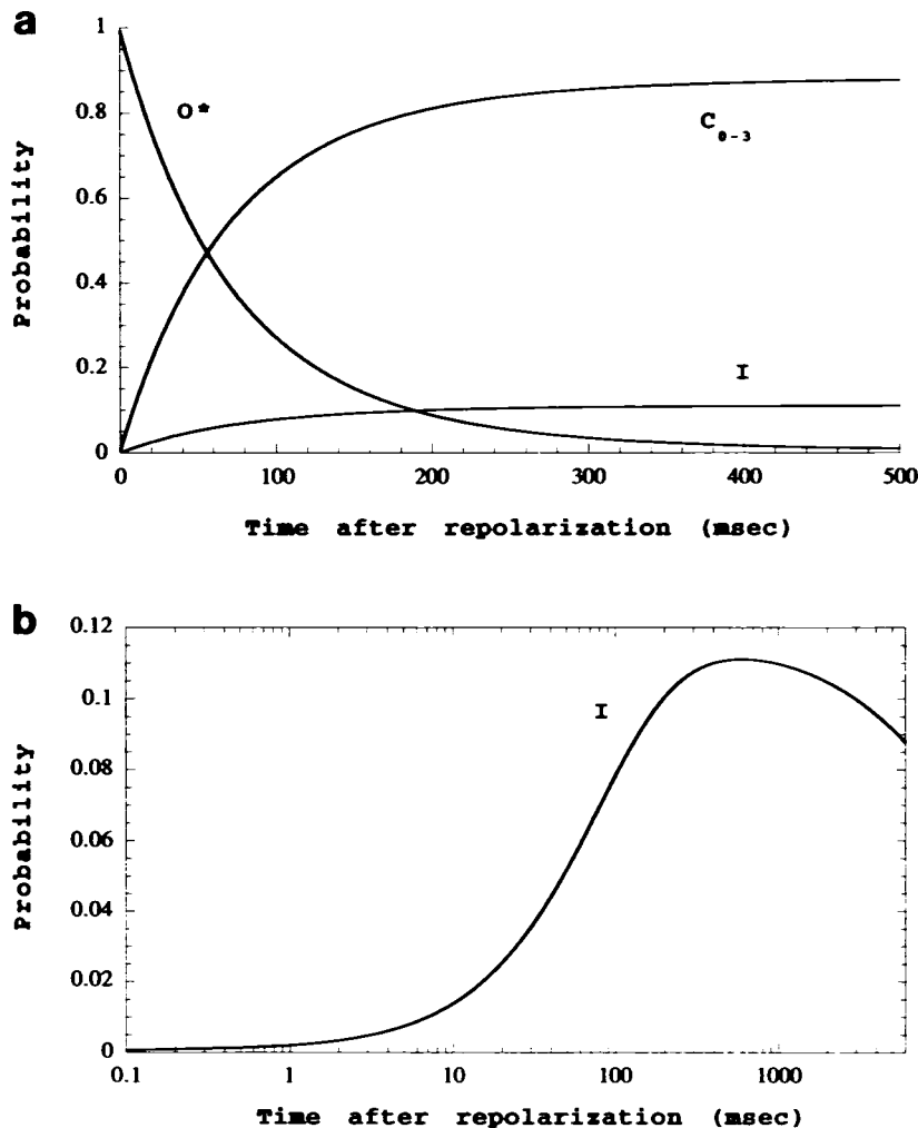
FIGURE 5 A simulation of the partitioning process as a function of interpulse duration. (a) A pool of activated channels ( O^* ) is allowed to partition between inactivated ( I ) and four deactivated ( C^* ) states during the interpulse. At t = 0 , O^* = 1 . Interpulse voltage is -80 mV. Note that although most of the channels occupy the deactivated states, a small but significant fraction accumulates in the inactivated state. Parameters for the model were derived as follows: Activation was fit to I_k(t) = \alpha(1 - \exp[-t/\tau_a])^4 and tail currents to I_k(t) = \alpha \exp[-4t/\tau_a] . Time constants for these relaxations were fit to rate equations,
